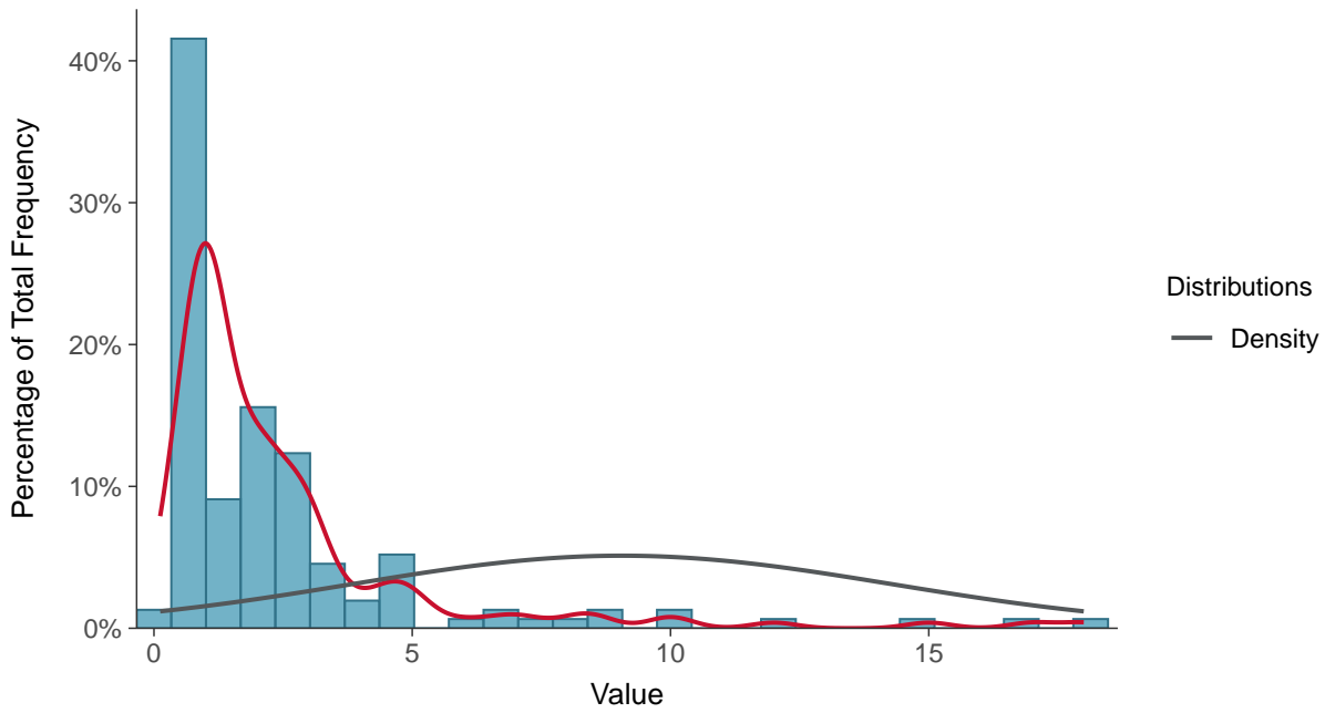
Arsenic, Pooled Background (ug/L)
